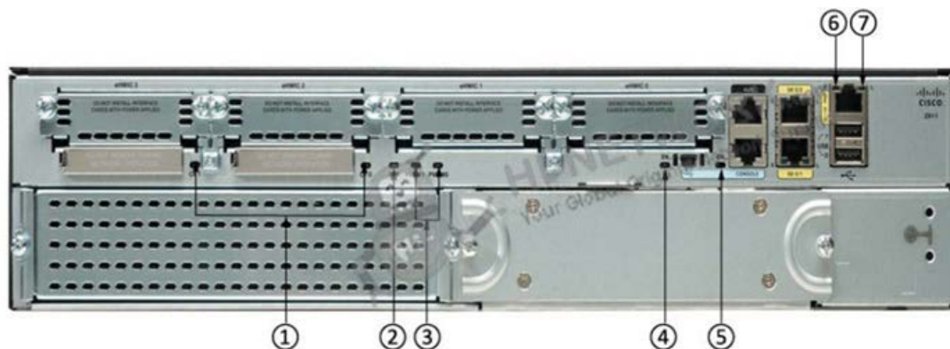
Figure 3 shows the LEDs on the back panel of CISCO2911-SEC/K9.
