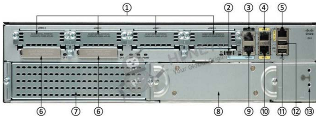
Figure 2 shows the ports on the back panel of CISCO2911-SEC/K9.
